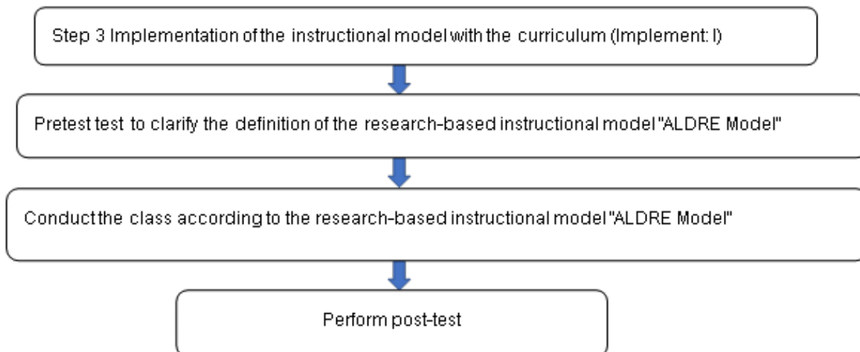
Figure 3: Step 3 Implementation
